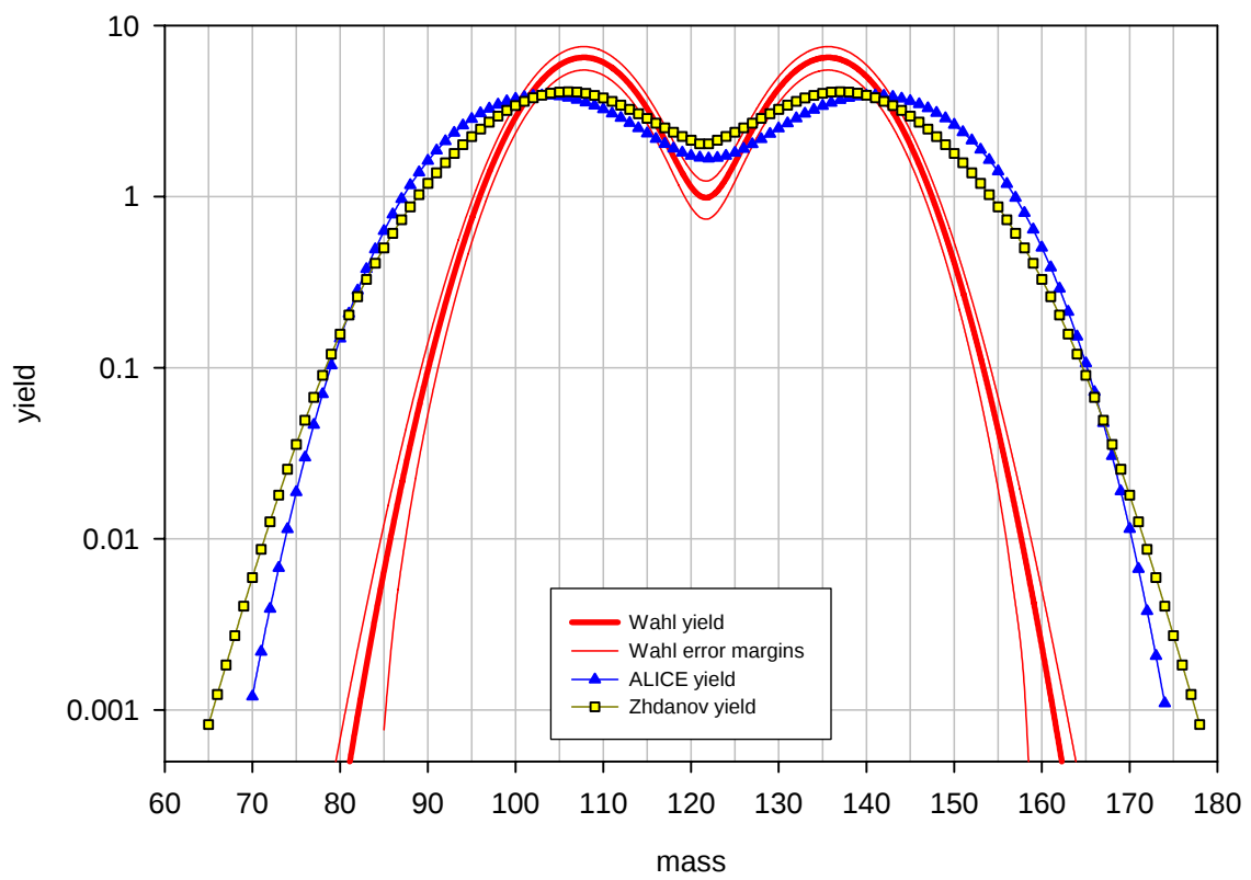
Benchmark B: ^{244}\text{Cm} at 28 MeV, pre-neutron emission mass distribution
